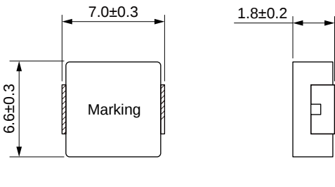
Dimensions: [mm]
